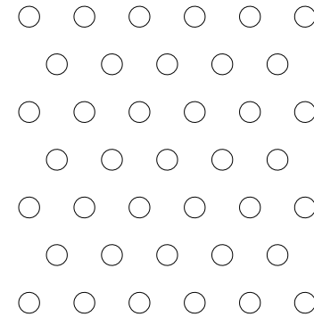
R18-216SG13 1/8" HOLES ON 21/64" STAGGERED CENTERS 13% OPEN AREA
