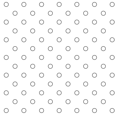
R564-732DG10 5/64" HOLES ON 7/32" DIAGONAL CENTERS 10% OPEN AREA
